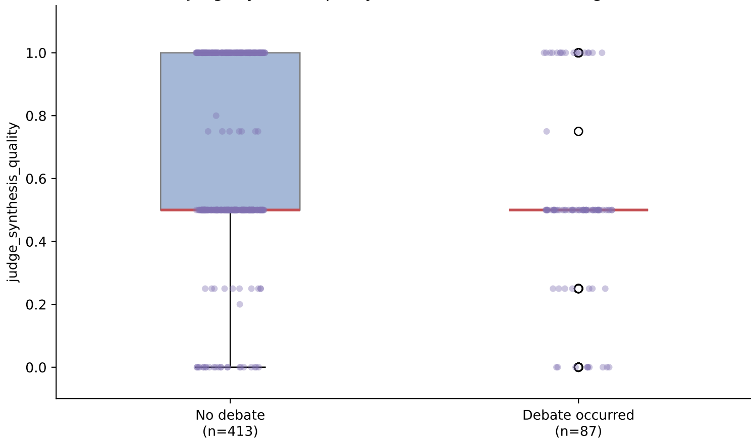
Judge synthesis quality: debate vs. no-debate images
